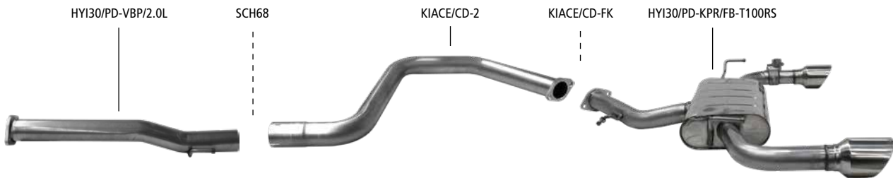
| Hyundai i30 Fastback N 2.0 T-GDI Performance | sports exhaust system after particulate filter | rear silencer with simple tailpipe 1x Ø 100mm LH+RH (RACE look), cut obliquely at 30°, for the original exhaust flap |
