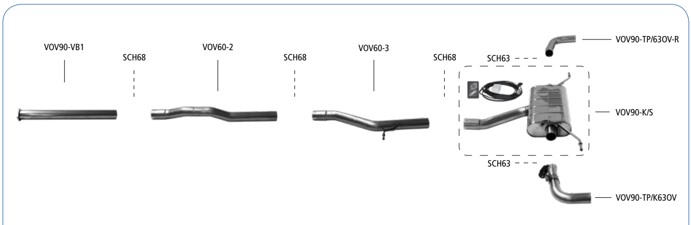
| Volvo V90 T6 AWD | sports exhaust system after catalytic converter | rear silencer and tailpipes with 1x exit Ø 63 mm LH+RH with exhaust flap control |
